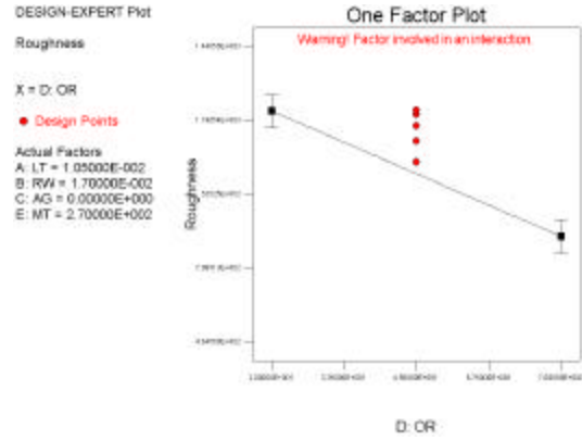
Figure 11 Plot of Surface Roughness Vs. Part Orientation
