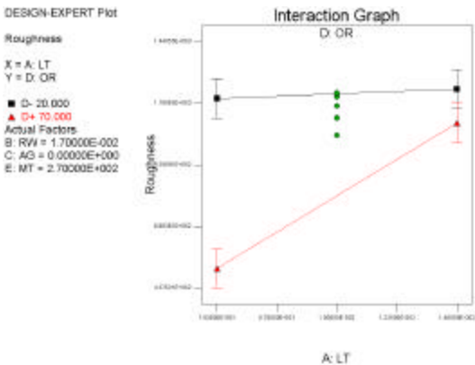
Figure 12 Interaction Plot of Surface Roughness Vs. Layer Thickness and Part Orientation
