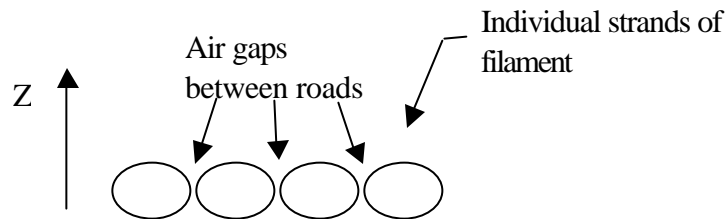
Figure 5 Cross-section of a layer showing roads and the air gap between roads
