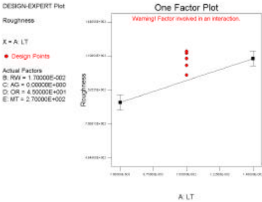
Figure 10 Plot of Surface Roughness Vs. Layer Thickness
